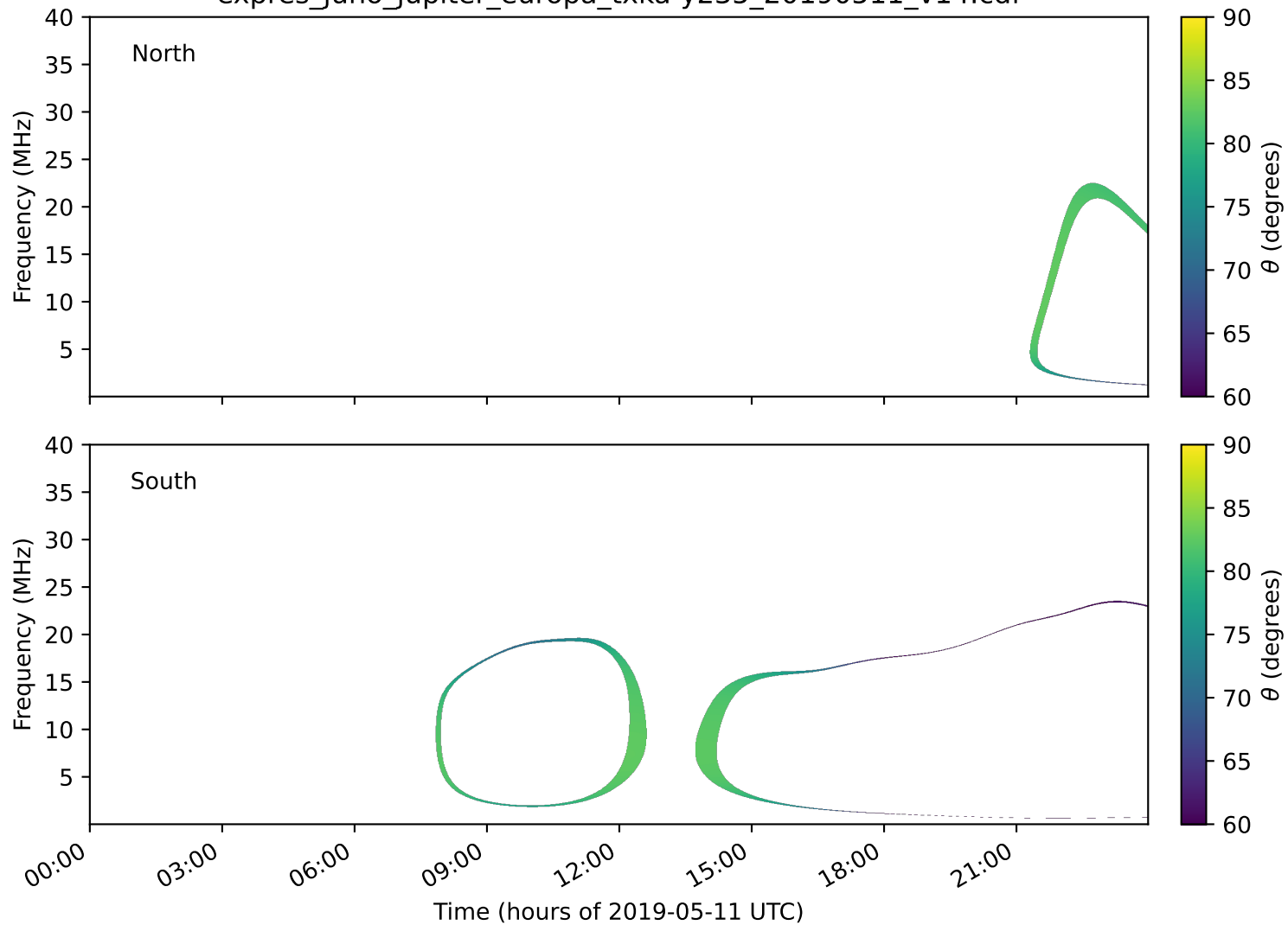
expres_juno_jupiter_europa_txka-y235_20190511_v14.cdf
