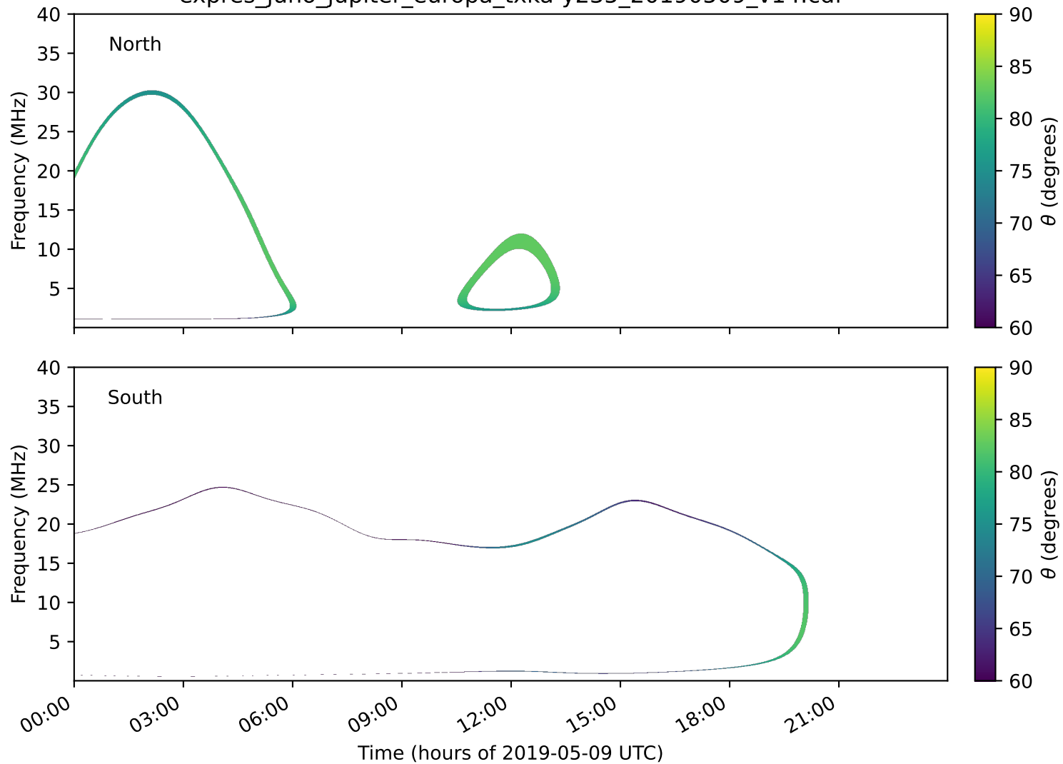
expres_juno_jupiter_europa_txka-y235_20190509_v14.cdf
