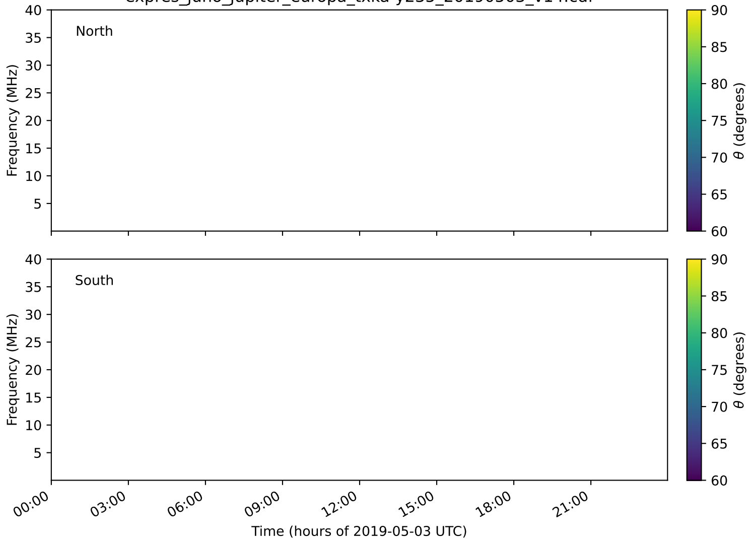
expres_juno_jupiter_europa_txka-y235_20190503_v14.cdf
