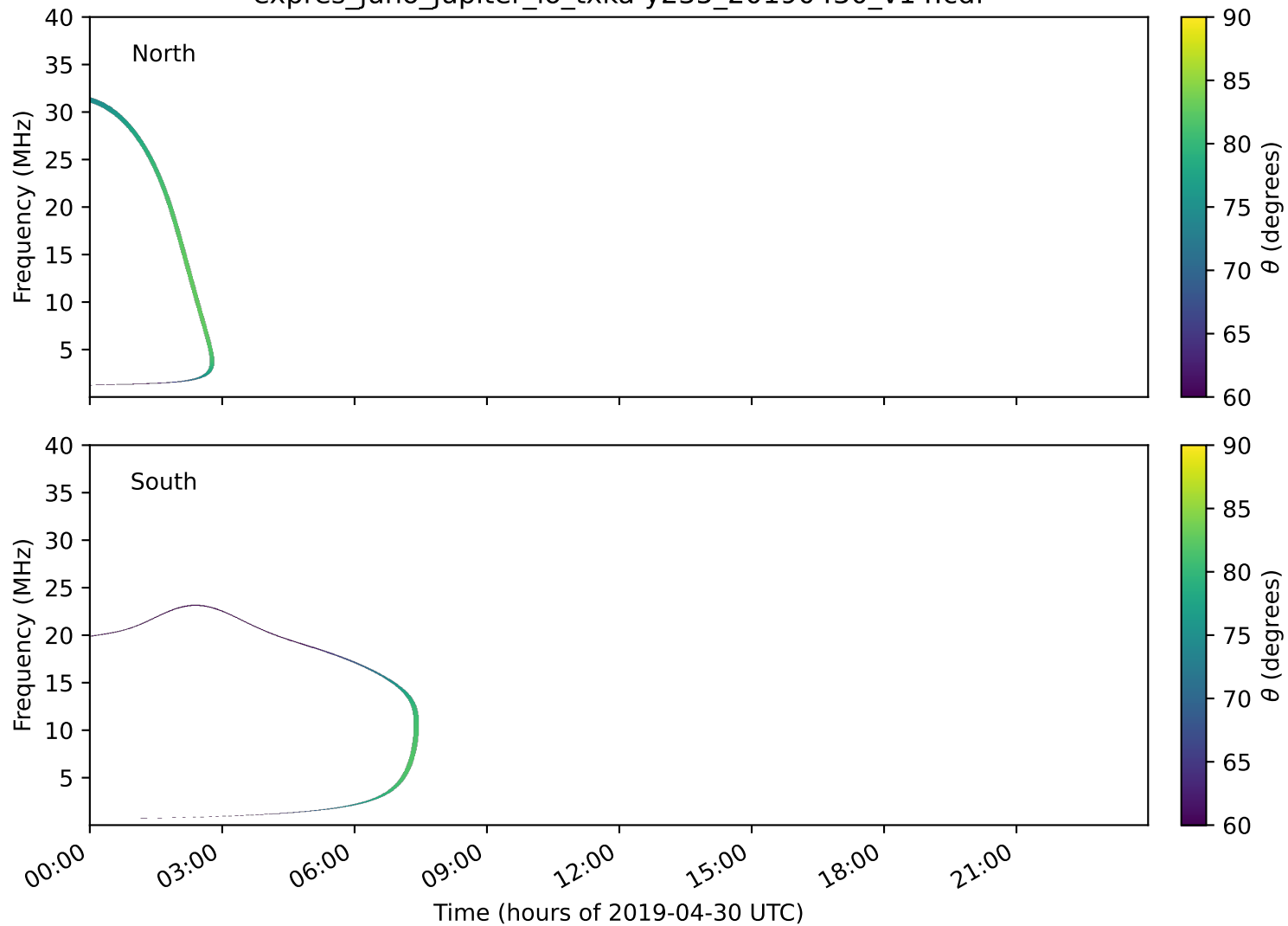
expres_juno_jupiter_io_txka-y235_20190430_v14.cdf
