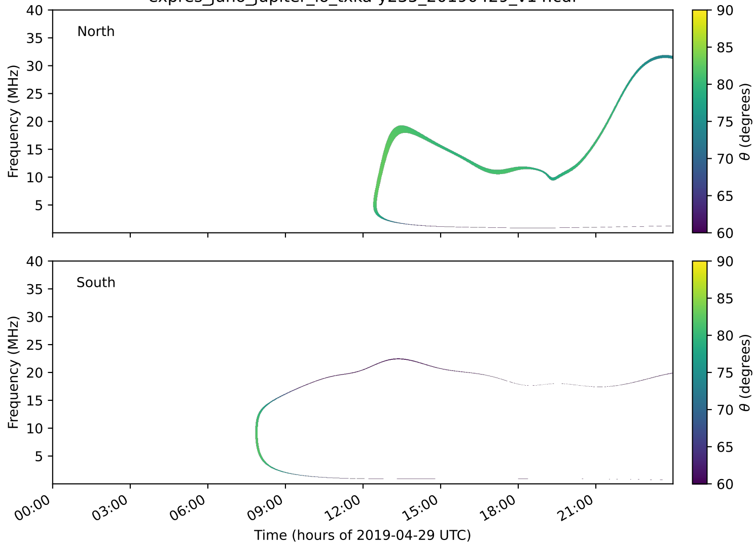
expres_juno_jupiter_io_txka-y235_20190429_v14.cdf
