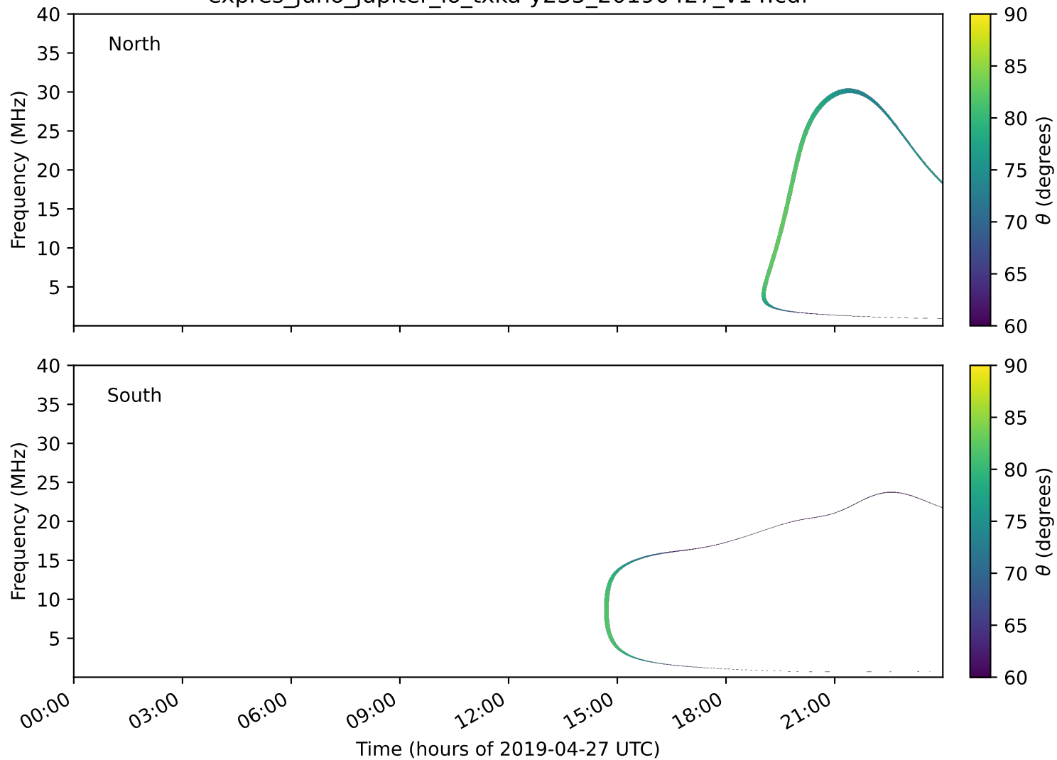
expres_juno_jupiter_io_txka-y235_20190427_v14.cdf
