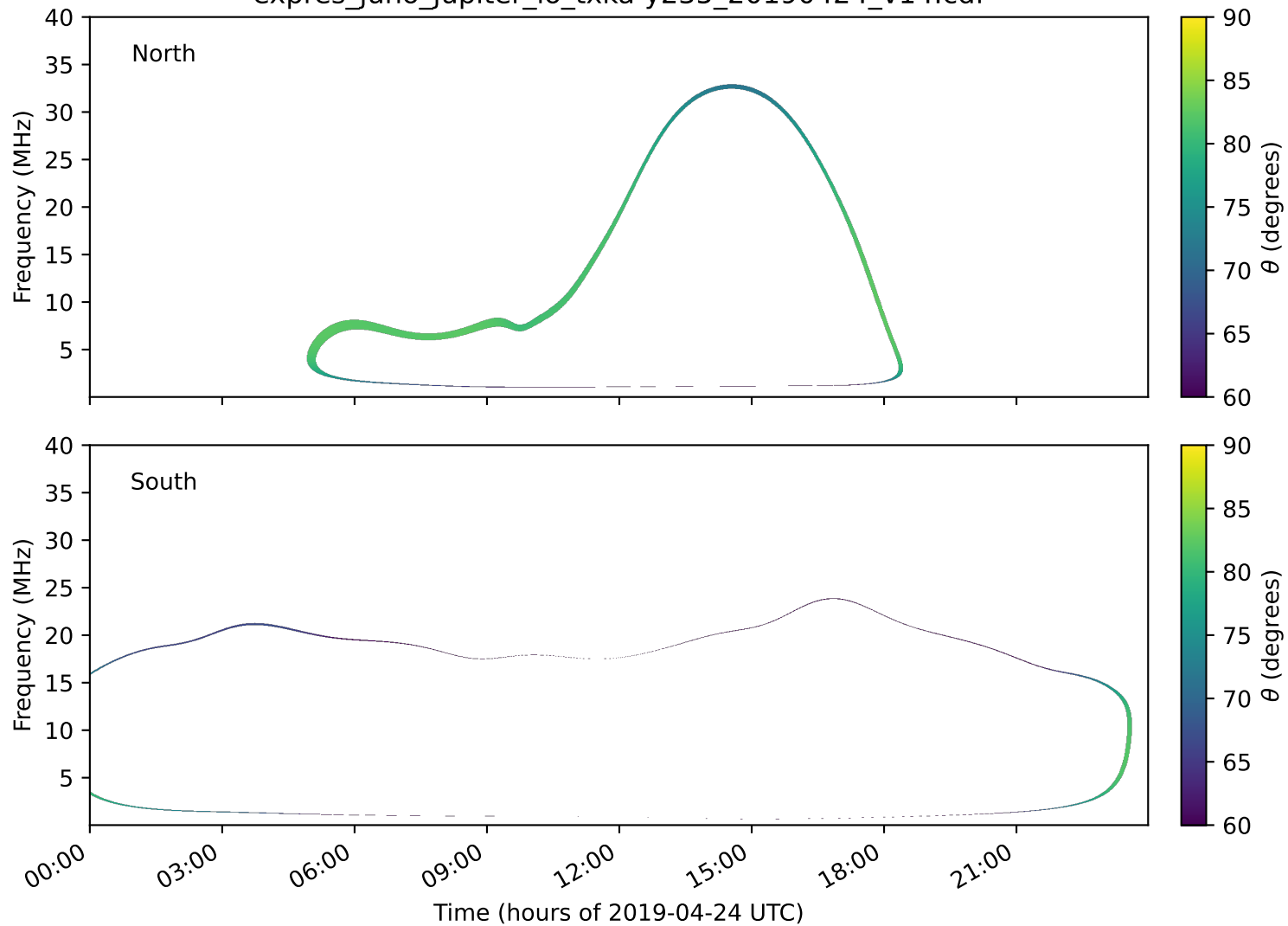
expres_juno_jupiter_io_txka-y235_20190424_v14.cdf
