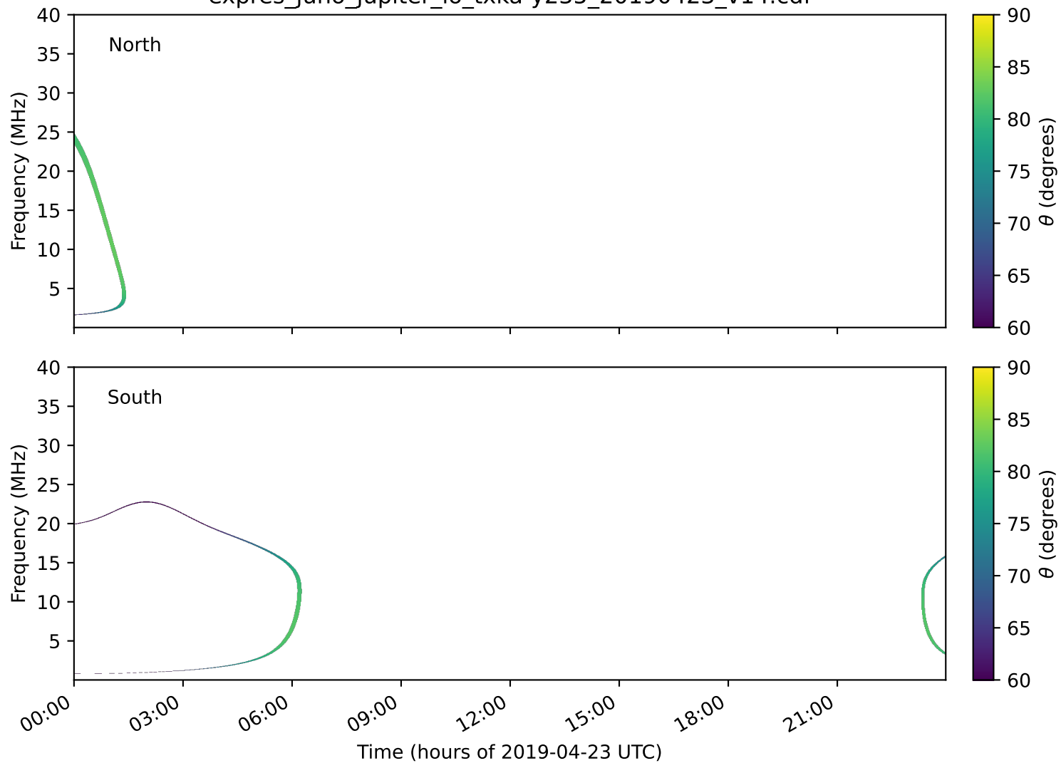
expres_juno_jupiter_io_txka-y235_20190423_v14.cdf
