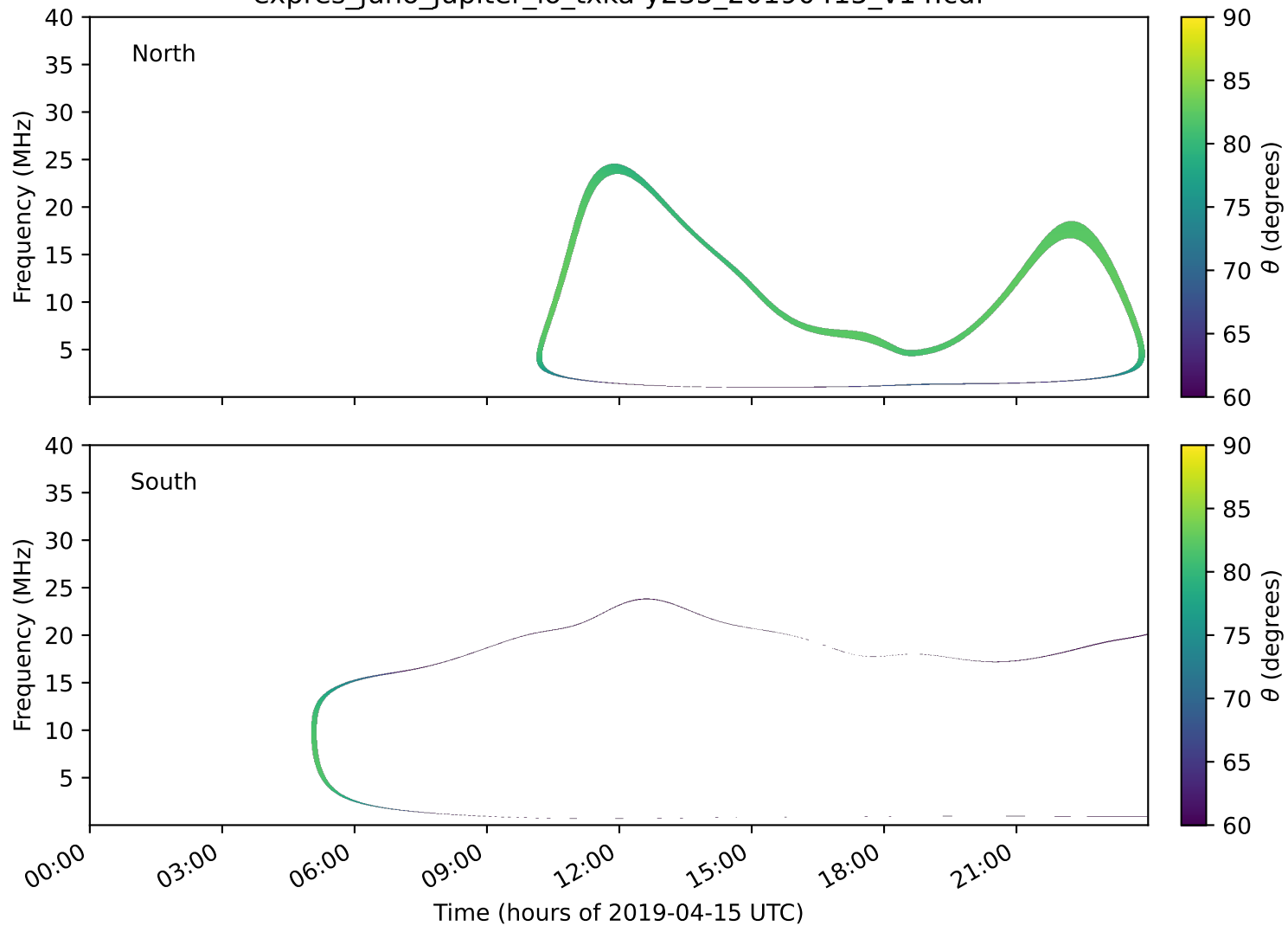
expres_juno_jupiter_io_txka-y235_20190415_v14.cdf
