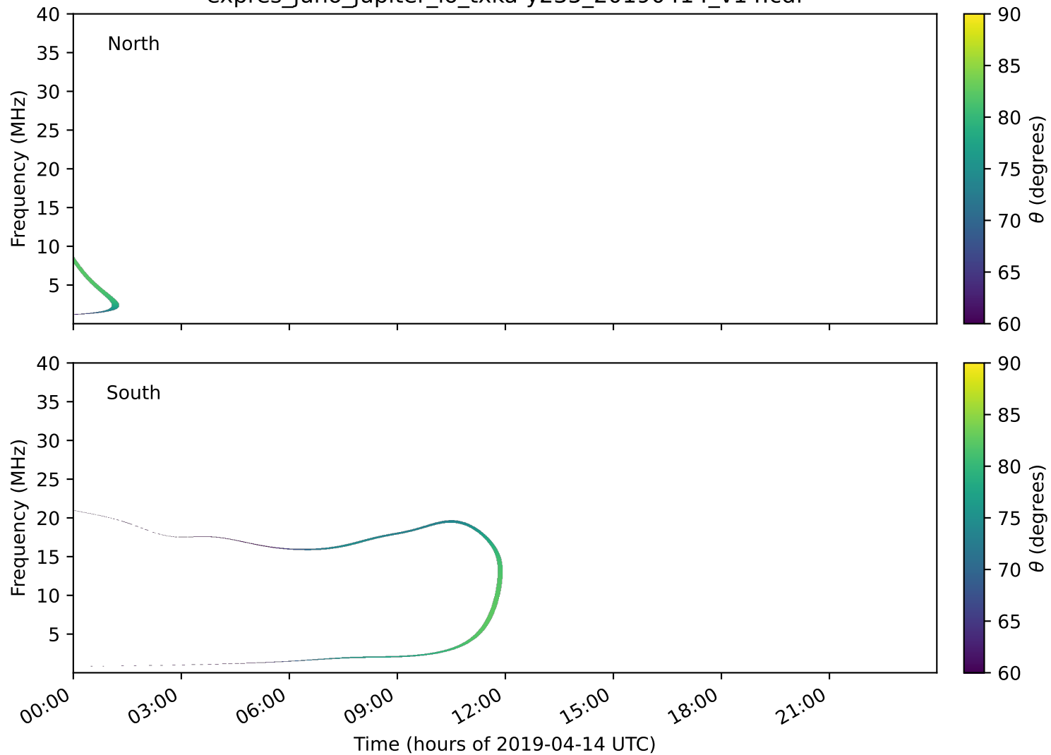
expres_juno_jupiter_io_txka-y235_20190414_v14.cdf
