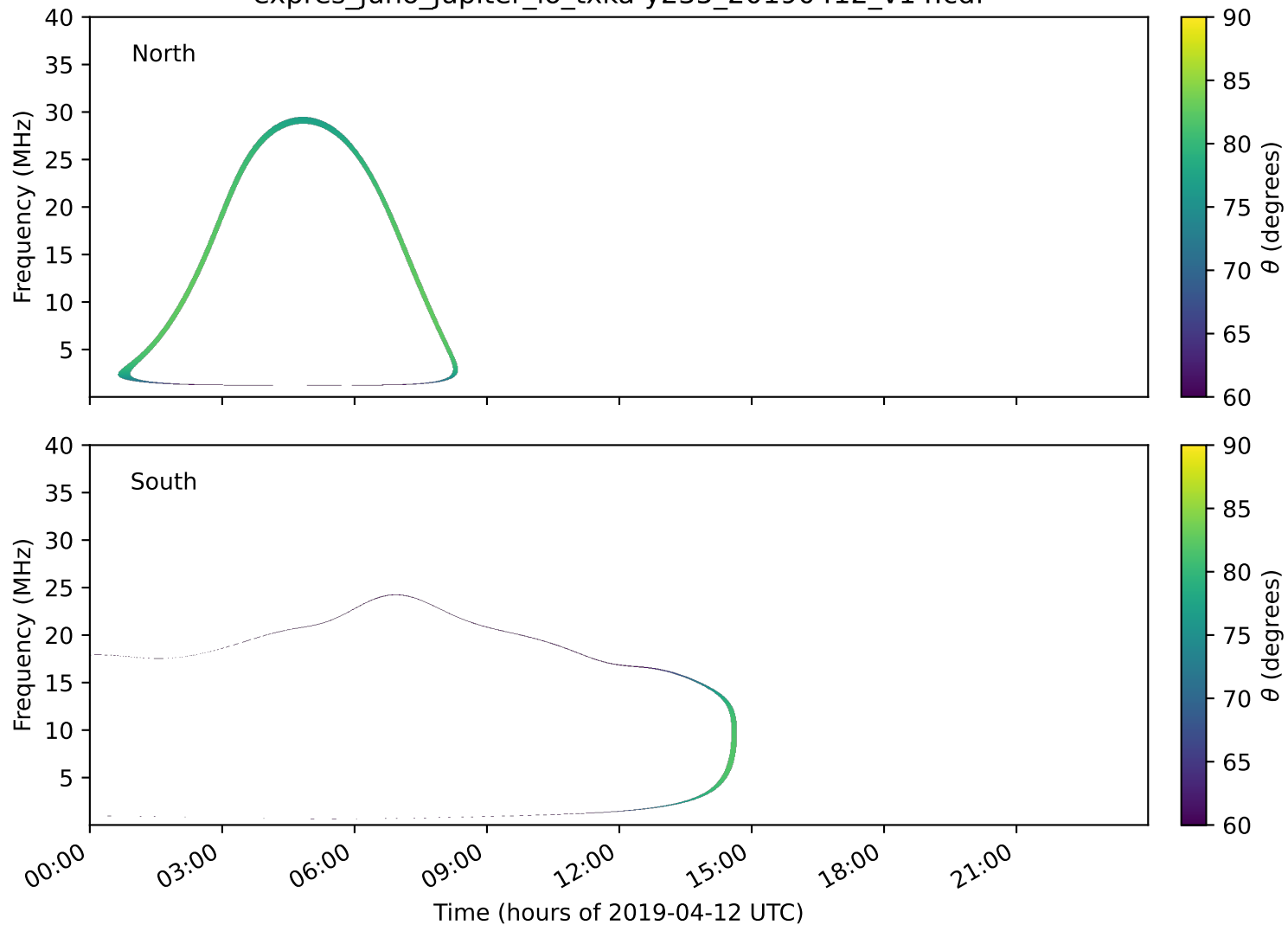
expres_juno_jupiter_io_txka-y235_20190412_v14.cdf
