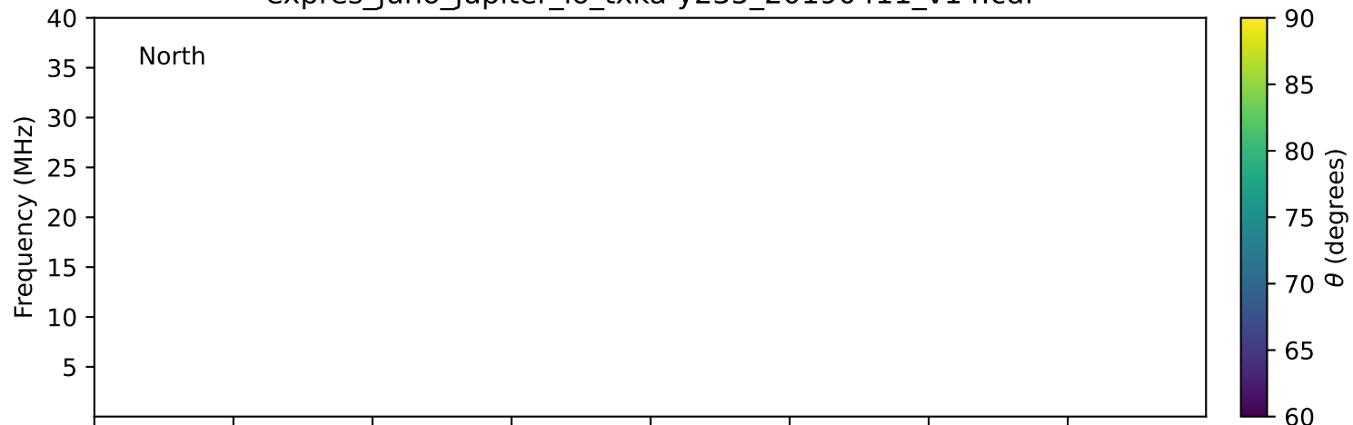
expres_juno_jupiter_io_txka-y235_20190411_v14.cdf
