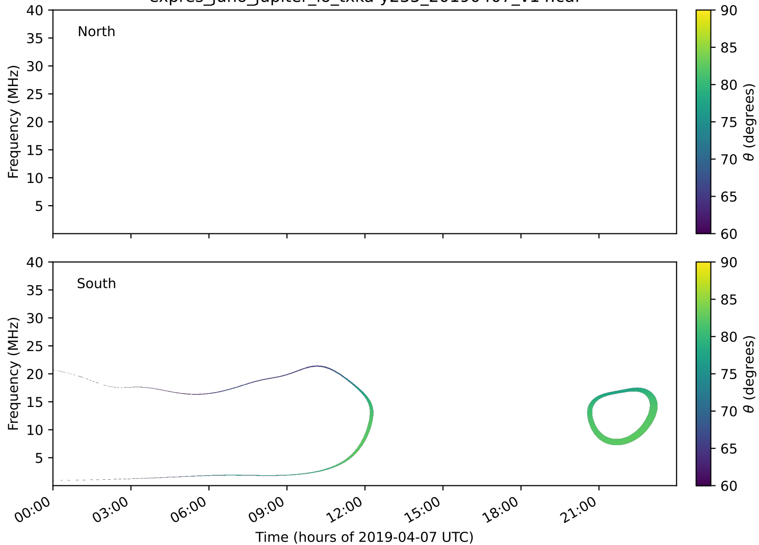
expres_juno_jupiter_io_txka-y235_20190407_v14.cdf
