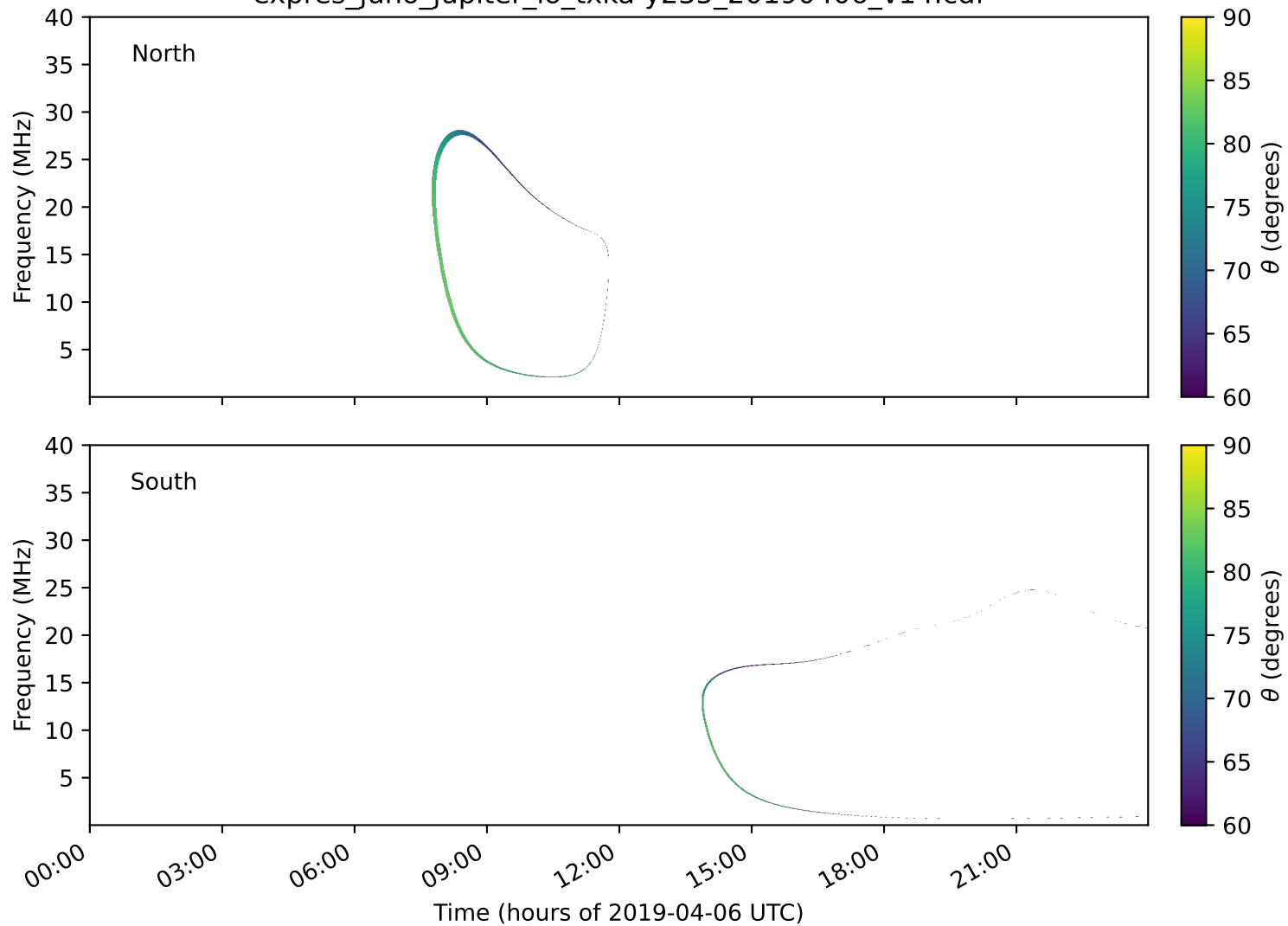
expres_juno_jupiter_io_txka-y235_20190406_v14.cdf
