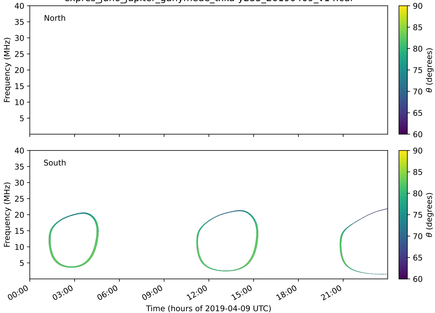
expres_juno_jupiter_ganymede_txka-y235_20190409_v14.cdf
