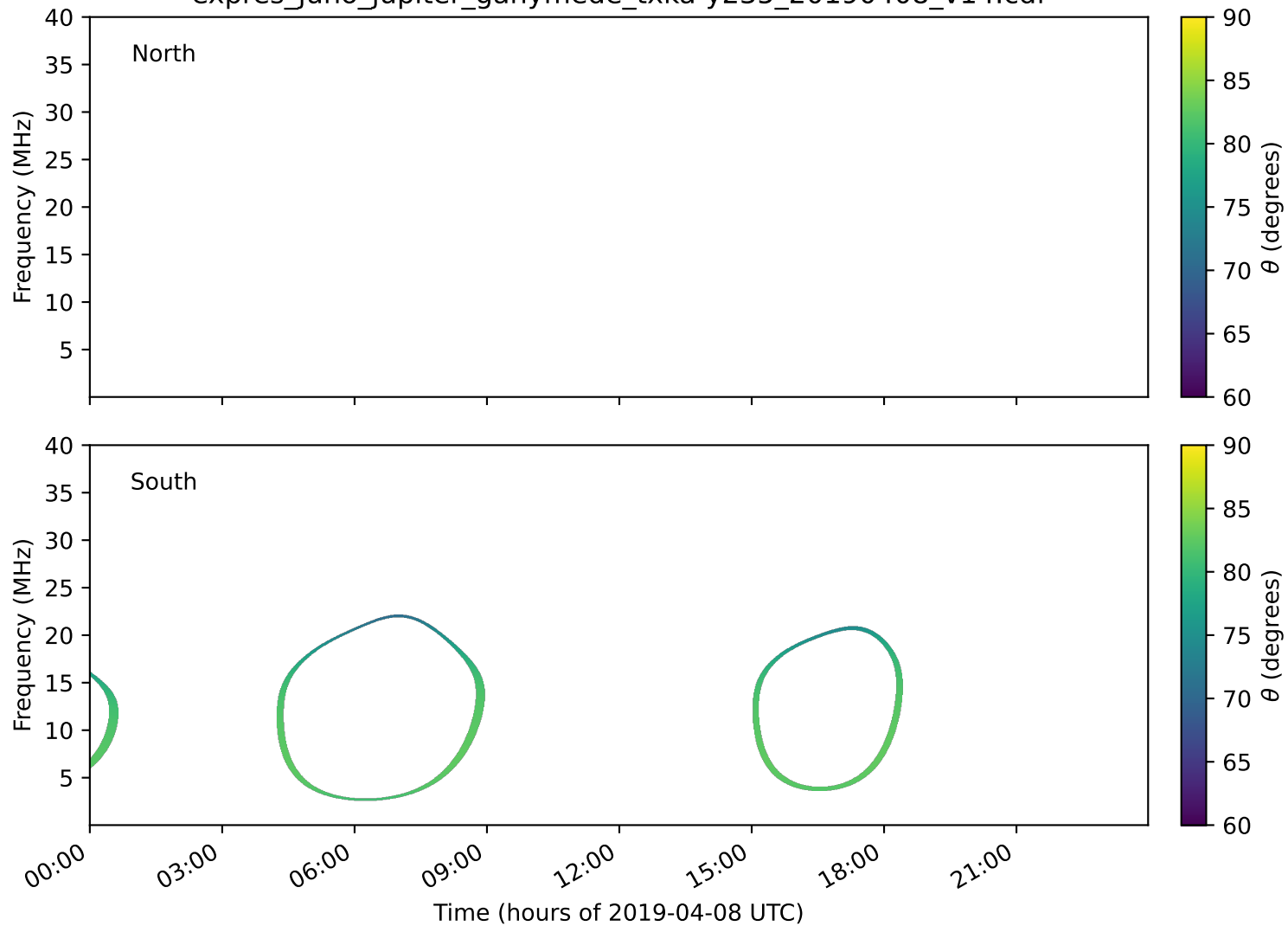
expres_juno_jupiter_ganymede_txka-y235_20190408_v14.cdf
