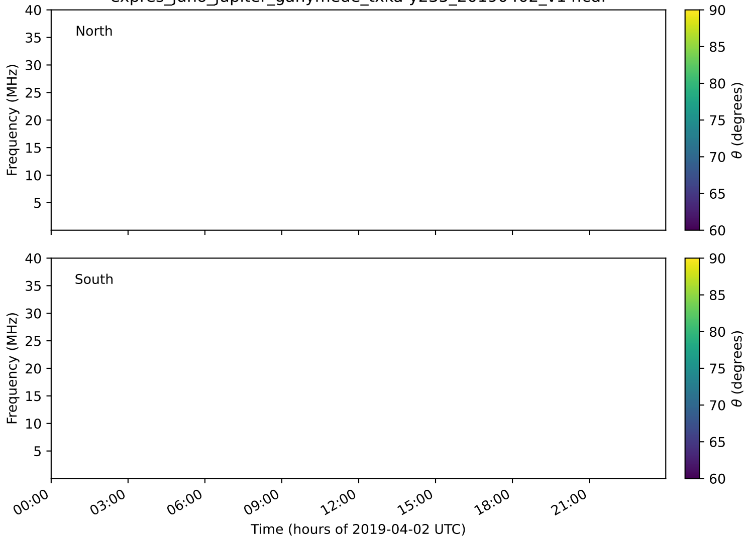
expres_juno_jupiter_ganymede_txka-y235_20190402_v14.cdf
