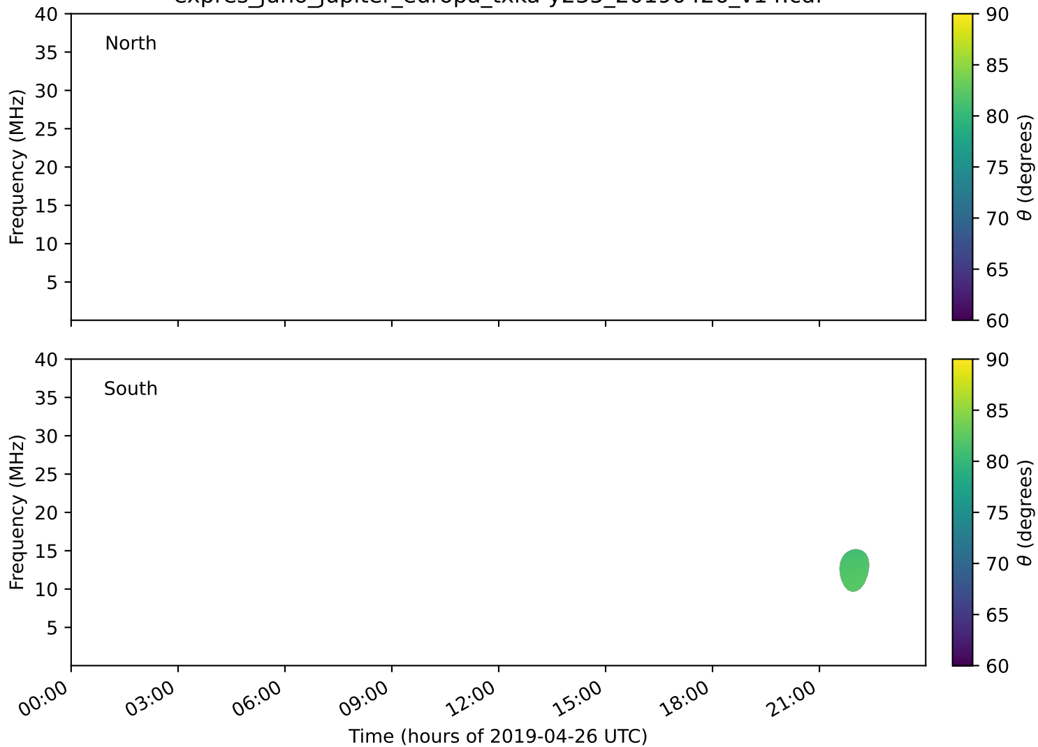
expres_juno_jupiter_europa_txka-y235_20190426_v14.cdf
