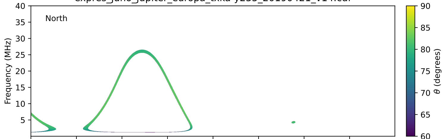
expres_juno_jupiter_europa_txka-y235_20190421_v14.cdf
