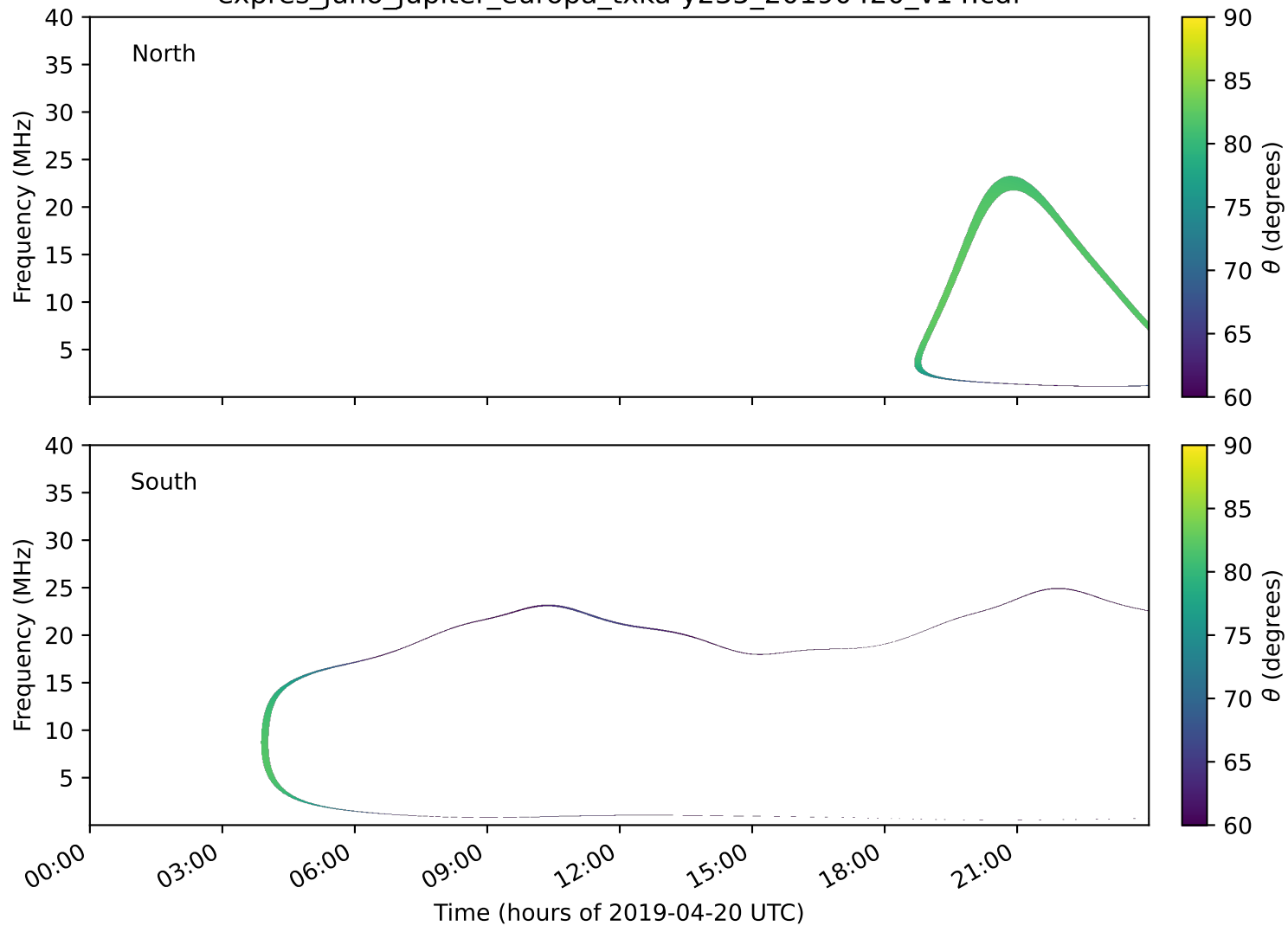
expres_juno_jupiter_europa_txka-y235_20190420_v14.cdf
