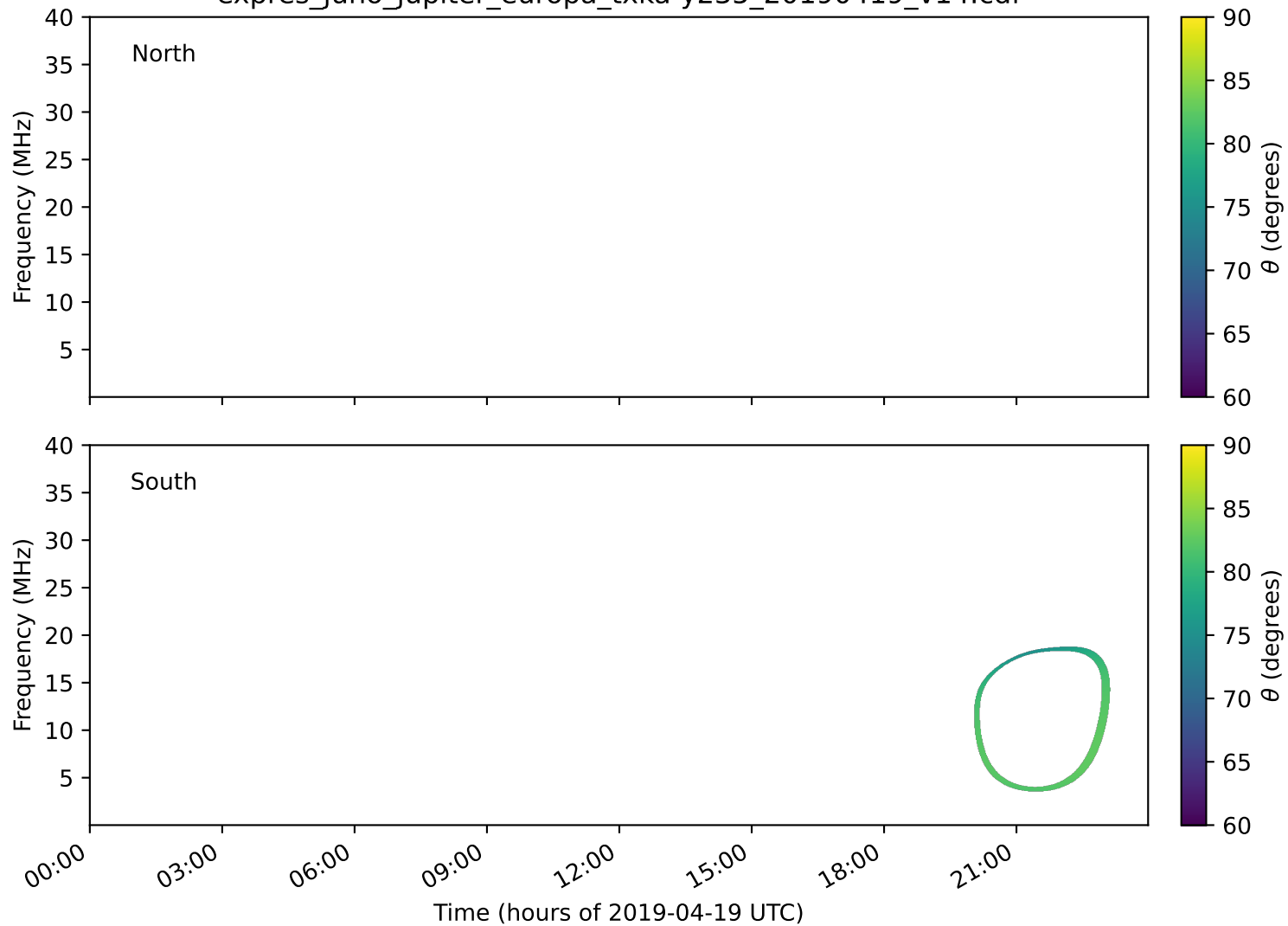
expres_juno_jupiter_europa_txka-y235_20190419_v14.cdf
