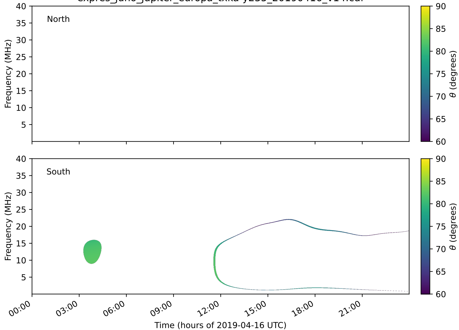
expres_juno_jupiter_europa_txka-y235_20190416_v14.cdf
