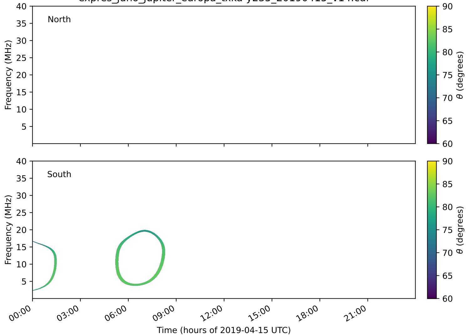
expres_juno_jupiter_europa_txka-y235_20190415_v14.cdf
