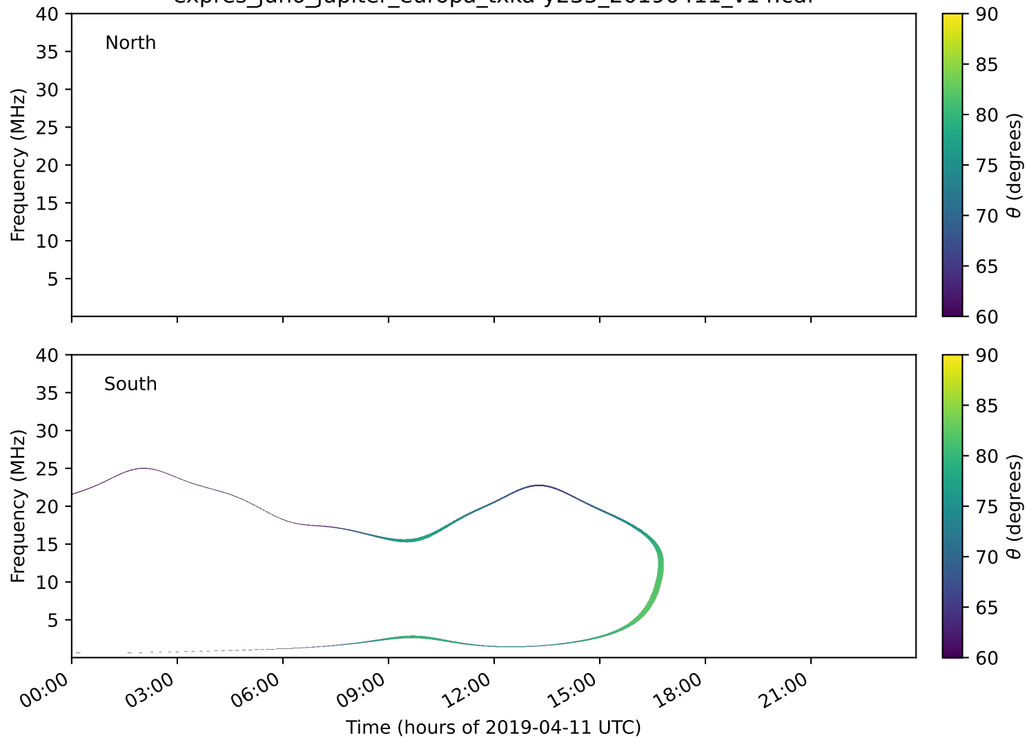
expres_juno_jupiter_europa_txka-y235_20190411_v14.cdf
