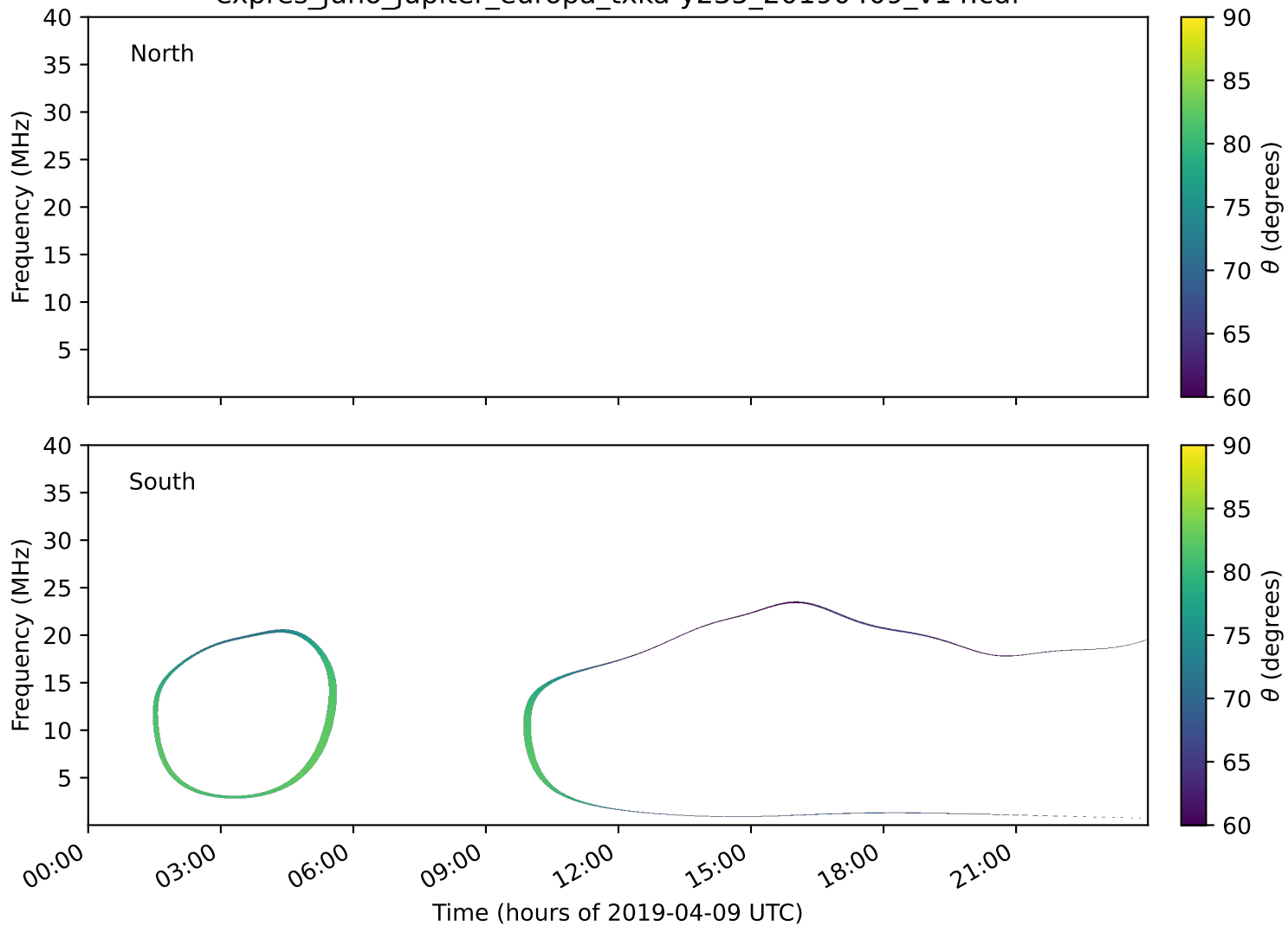
expres_juno_jupiter_europa_txka-y235_20190409_v14.cdf
