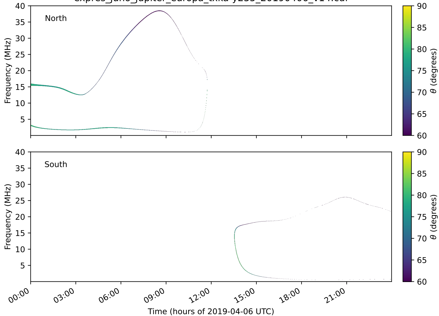
expres_juno_jupiter_europa_txka-y235_20190406_v14.cdf
