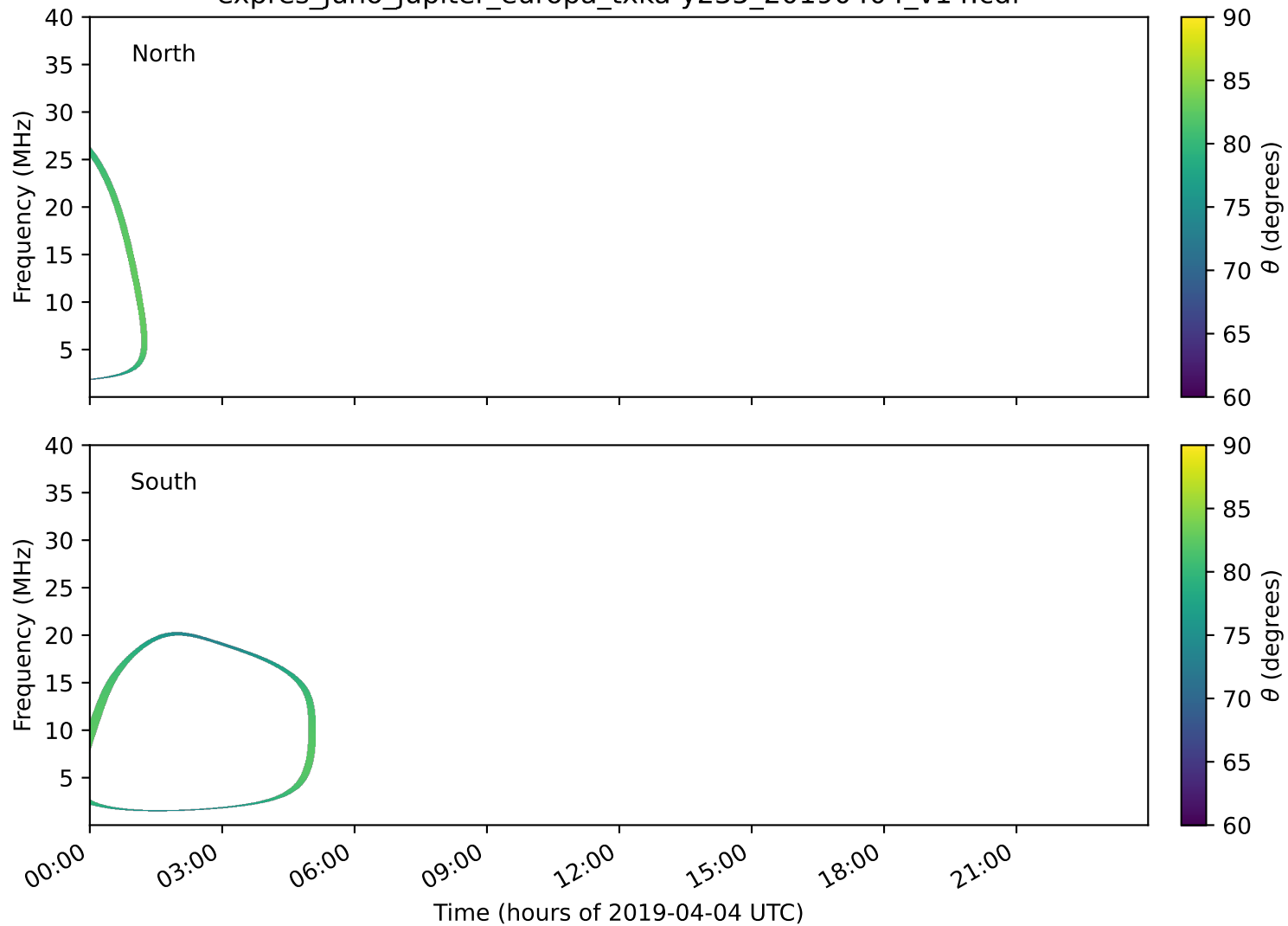
expres_juno_jupiter_europa_txka-y235_20190404_v14.cdf
