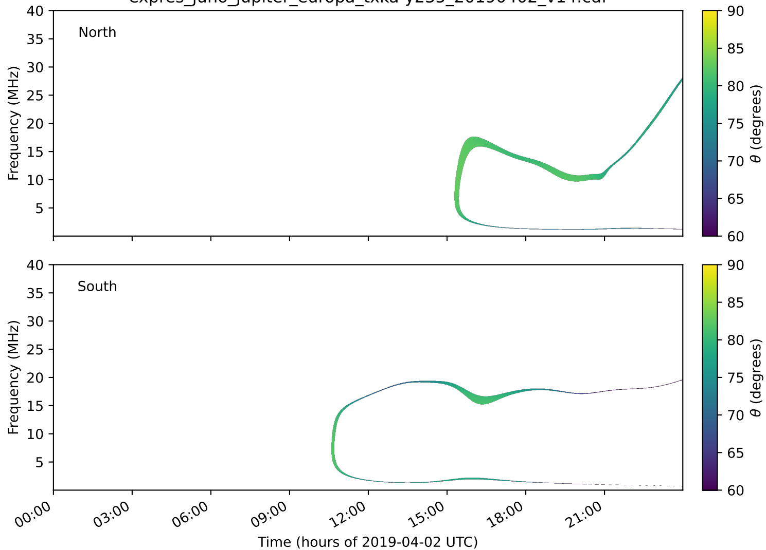
expres_juno_jupiter_europa_txka-y235_20190402_v14.cdf
