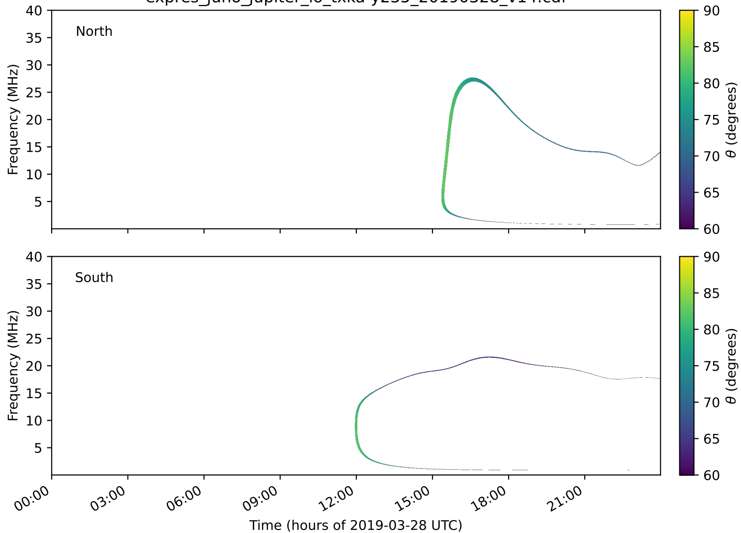
expres_juno_jupiter_io_txka-y235_20190328_v14.cdf
