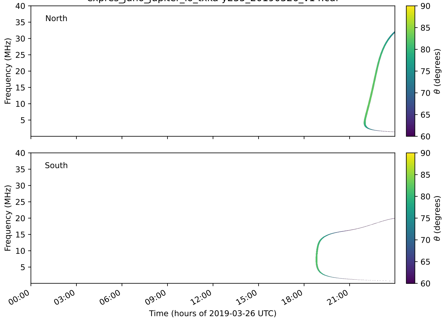
expres_juno_jupiter_io_txka-y235_20190326_v14.cdf
