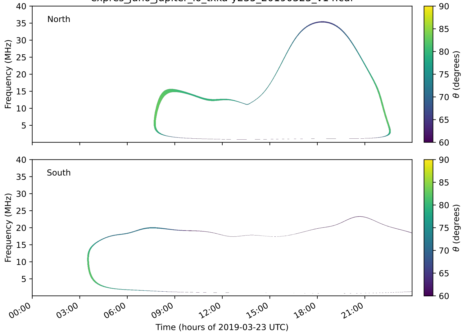
expres_juno_jupiter_io_txka-y235_20190323_v14.cdf
