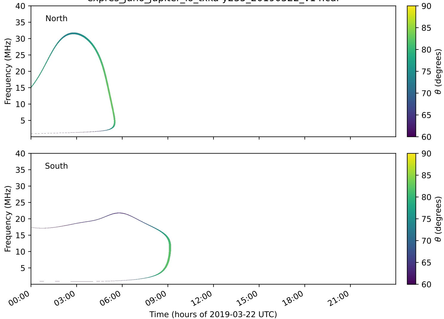
expres_juno_jupiter_io_txka-y235_20190322_v14.cdf
