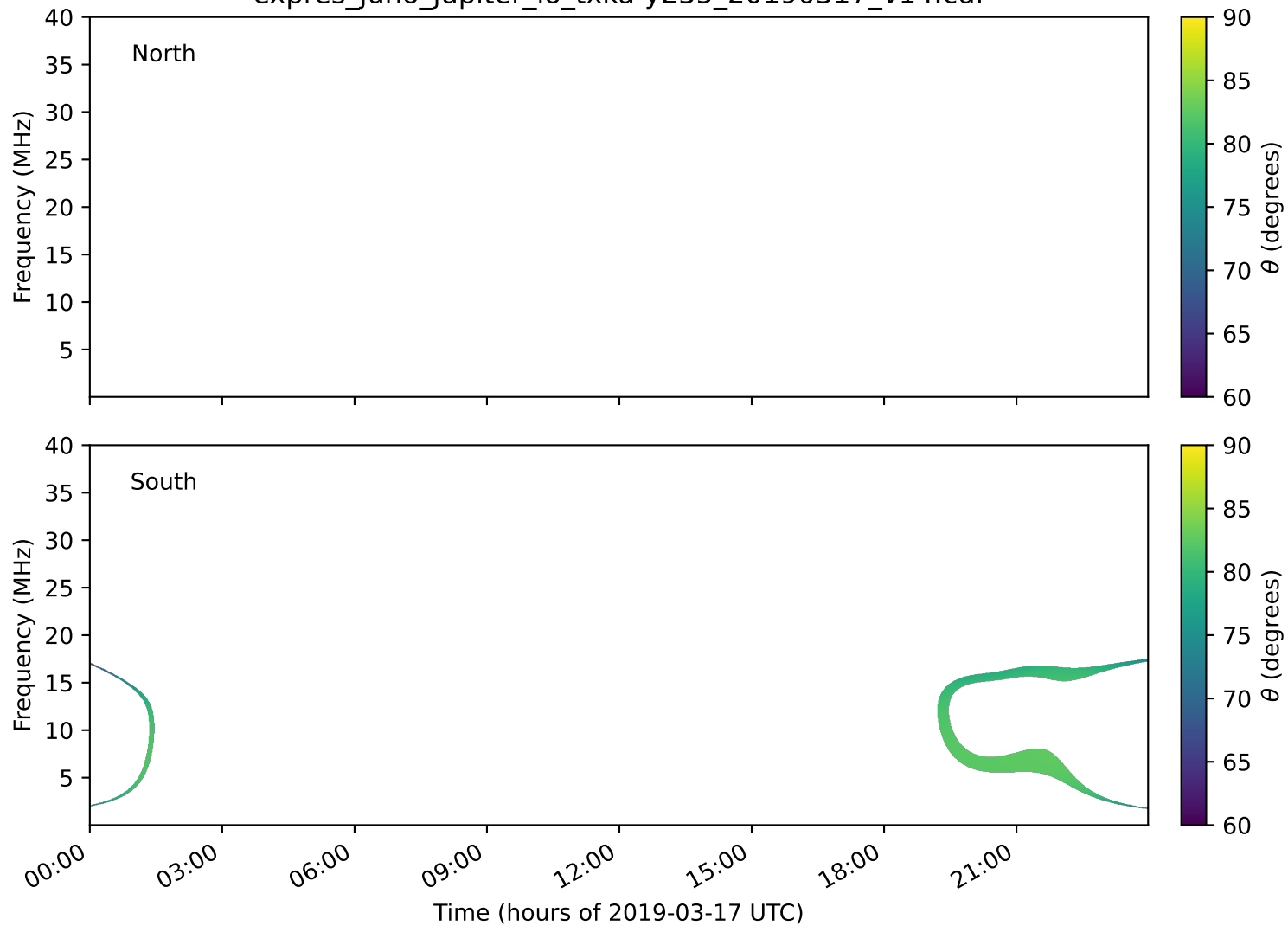
expres_juno_jupiter_io_txka-y235_20190317_v14.cdf
