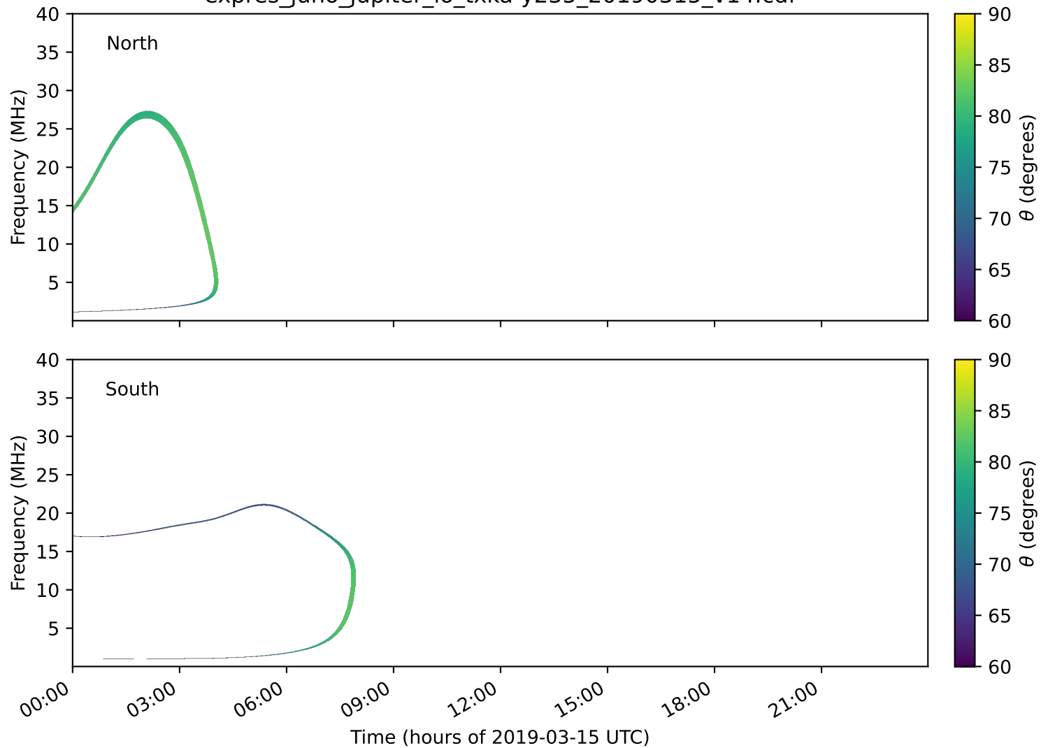
expres_juno_jupiter_io_txka-y235_20190315_v14.cdf
