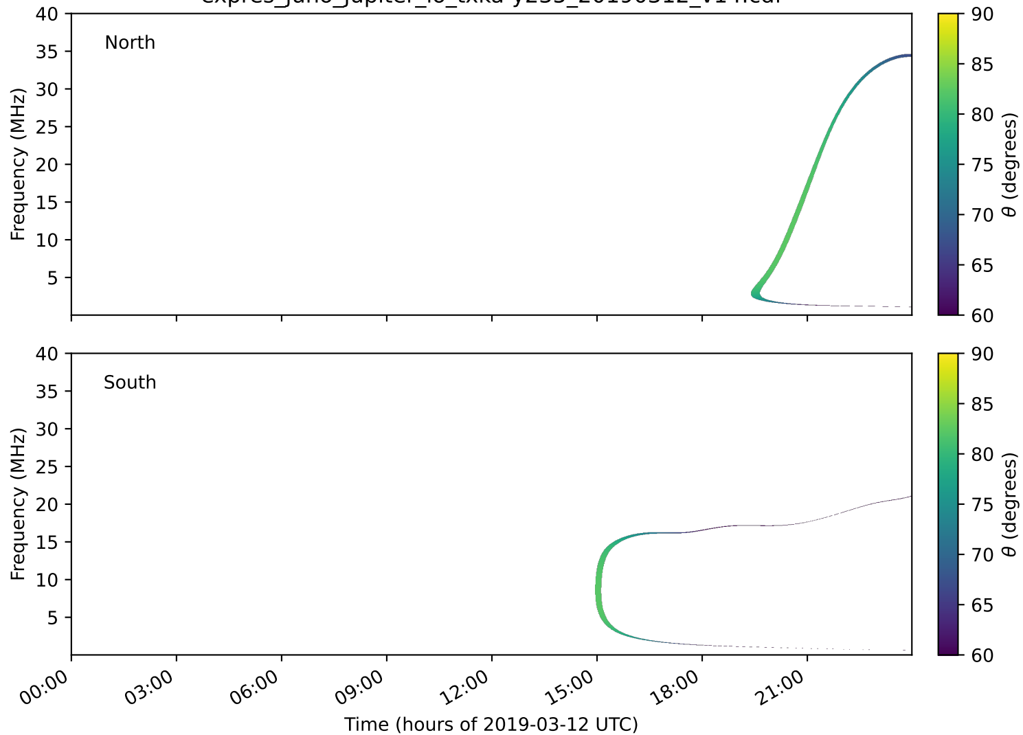
expres_juno_jupiter_io_txka-y235_20190312_v14.cdf
