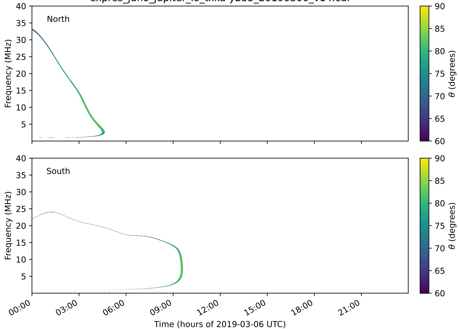
expres_juno_jupiter_io_txka-y235_20190306_v14.cdf
