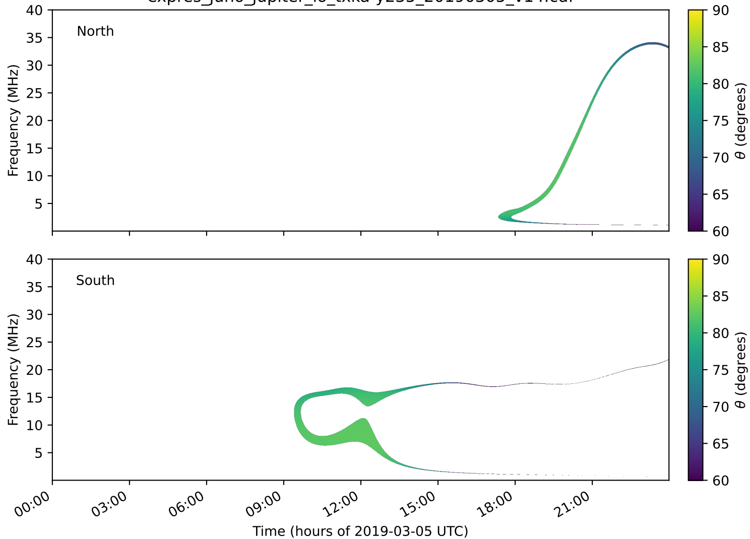
expres_juno_jupiter_io_txka-y235_20190305_v14.cdf
