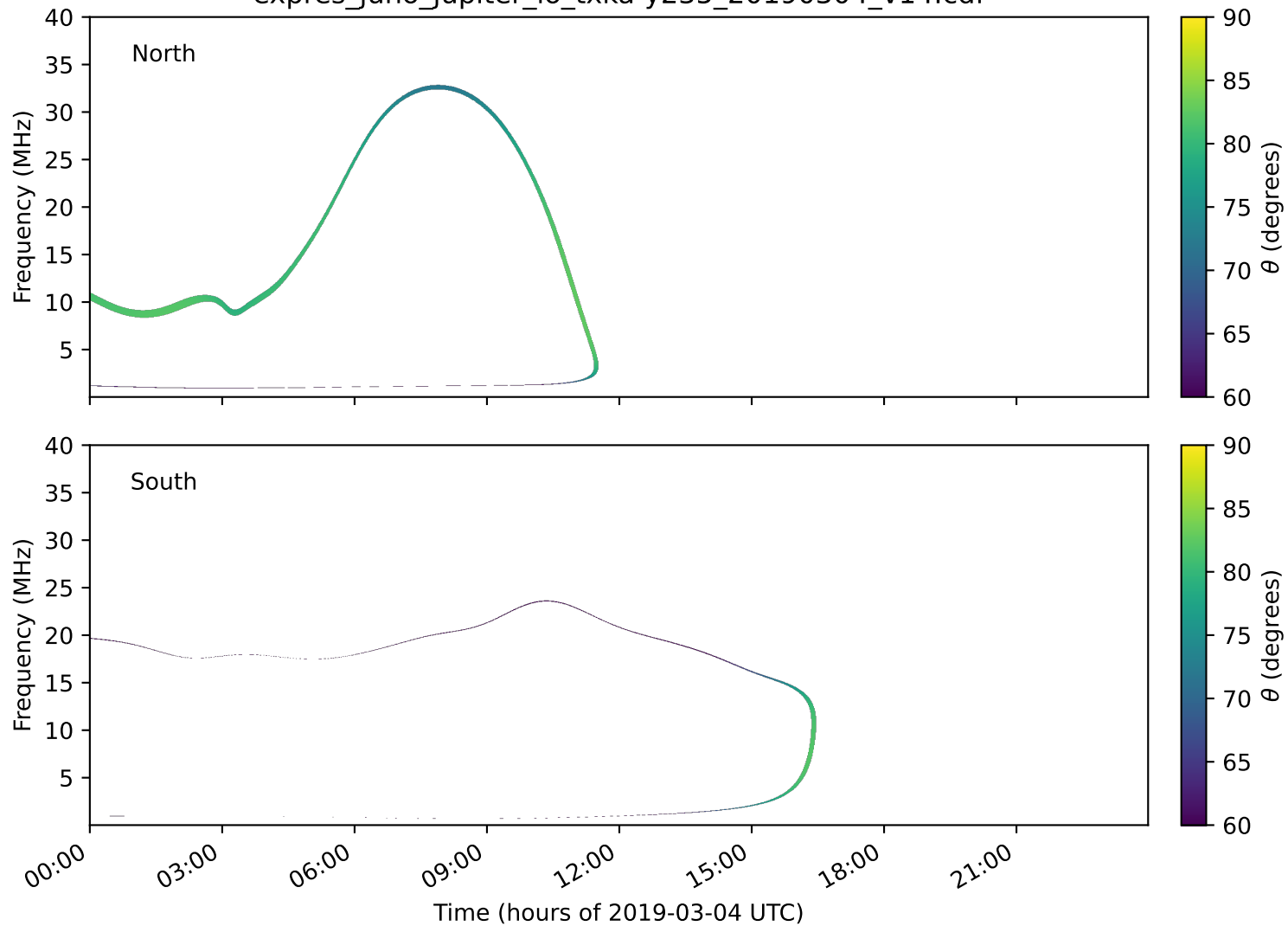
expres_juno_jupiter_io_txka-y235_20190304_v14.cdf
