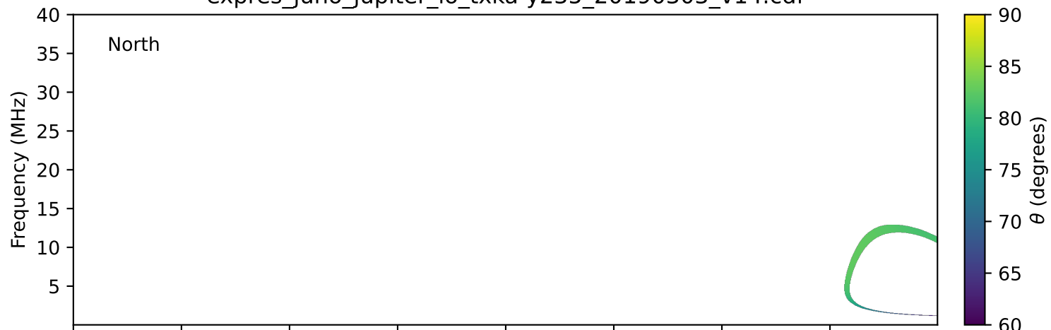
expres_juno_jupiter_io_txka-y235_20190303_v14.cdf
