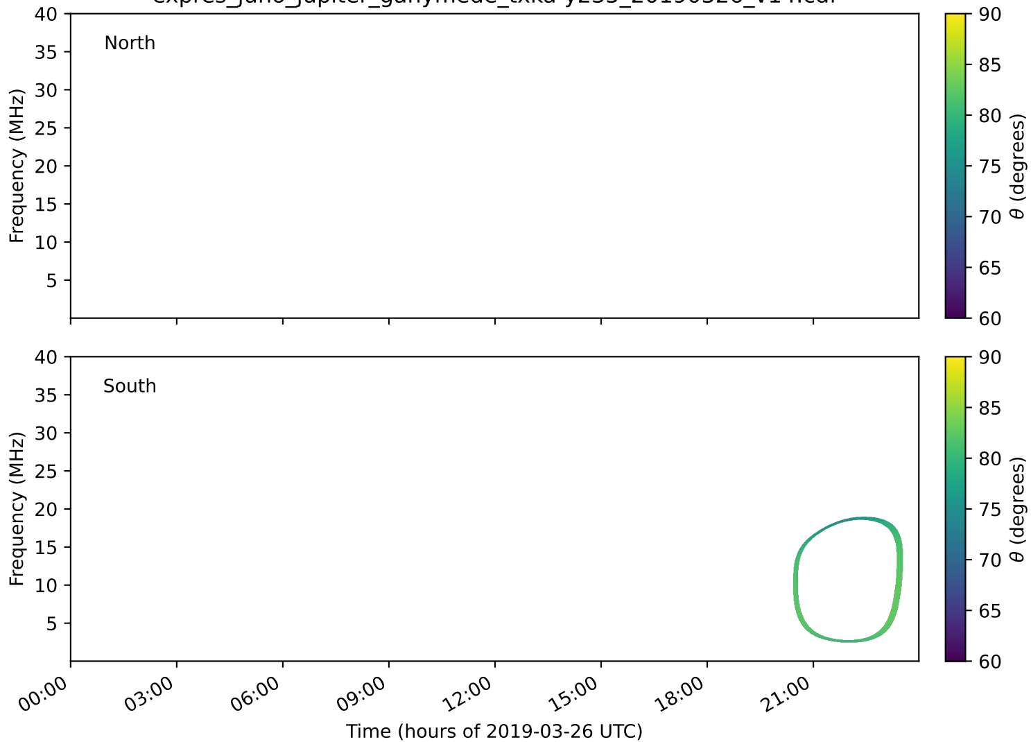
expres_juno_jupiter_ganymede_txka-y235_20190326_v14.cdf
