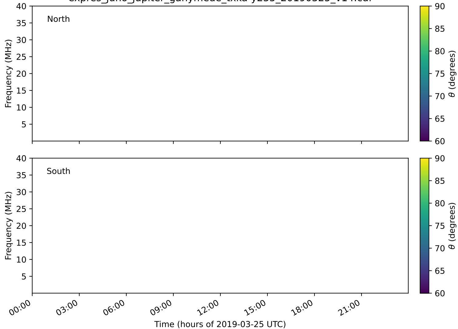
expres_juno_jupiter_ganymede_txka-y235_20190325_v14.cdf
