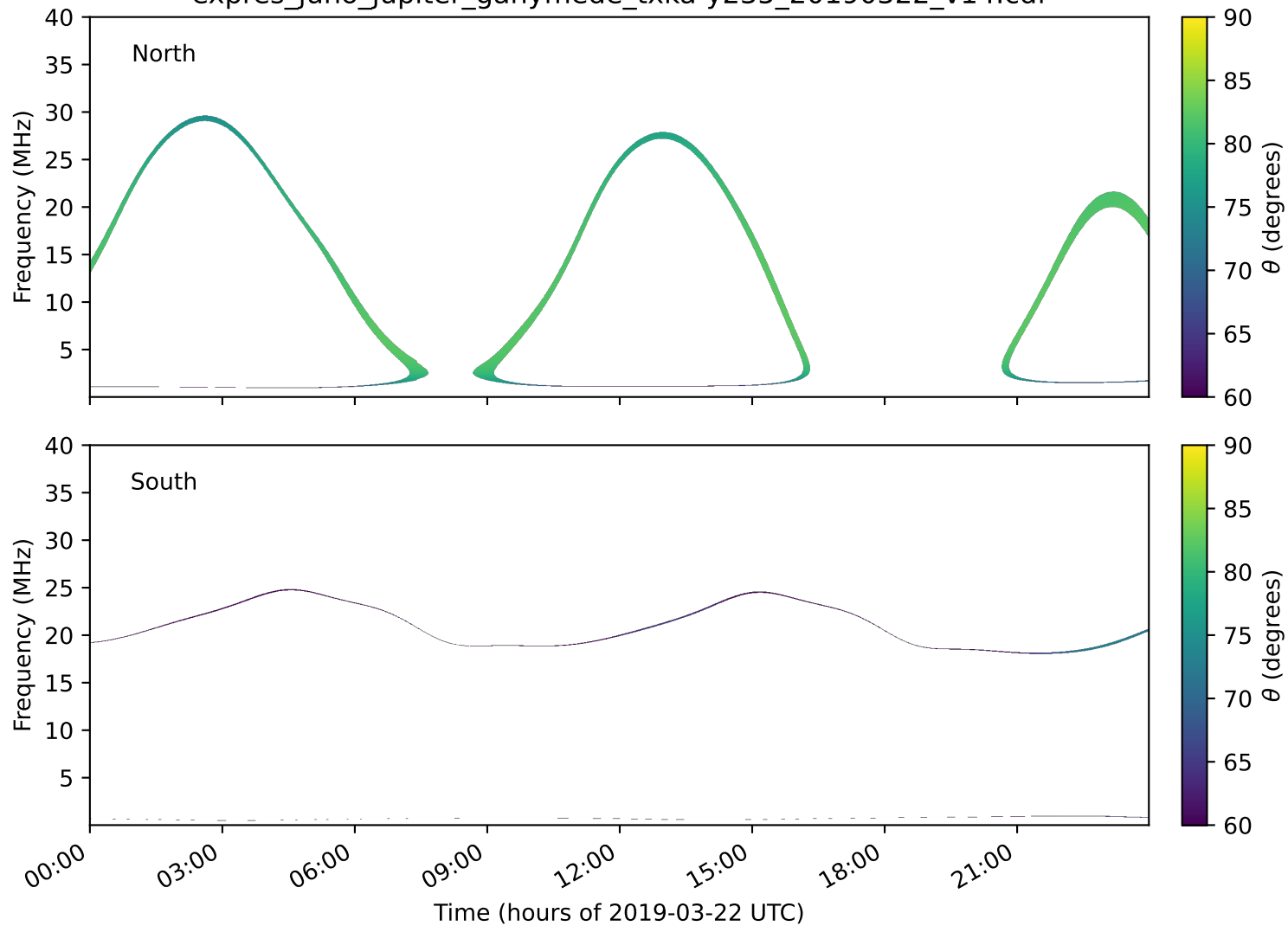
expres_juno_jupiter_ganymede_txka-y235_20190322_v14.cdf
