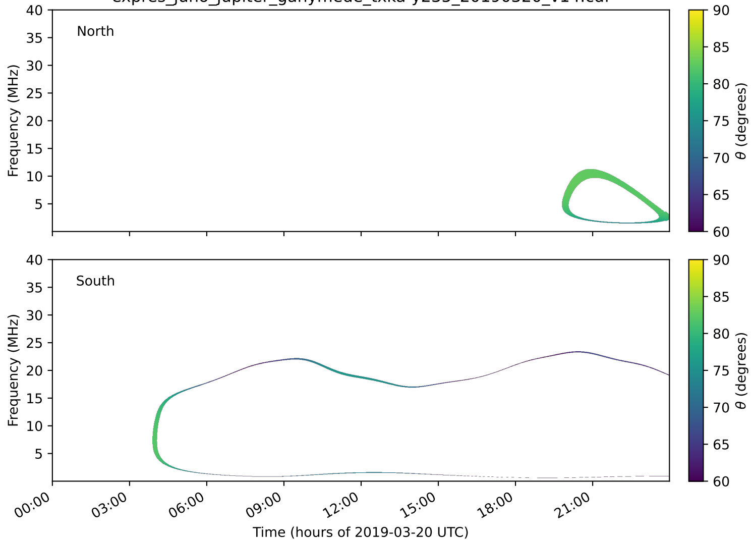
expres_juno_jupiter_ganymede_txka-y235_20190320_v14.cdf
