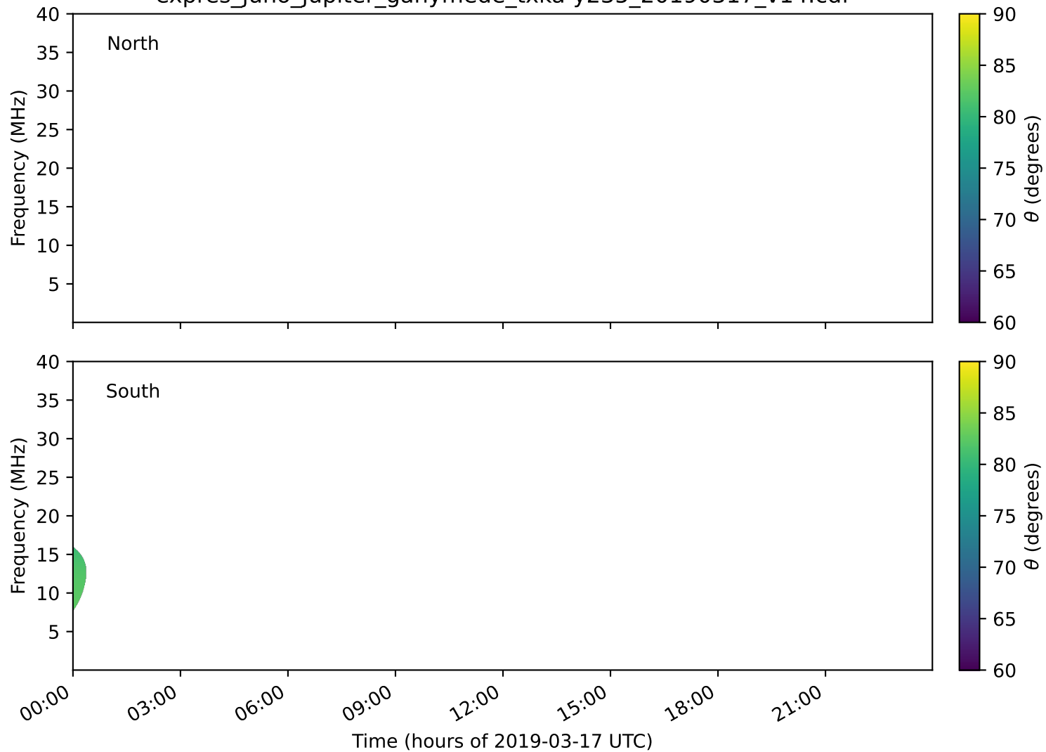
expres_juno_jupiter_ganymede_txka-y235_20190317_v14.cdf
