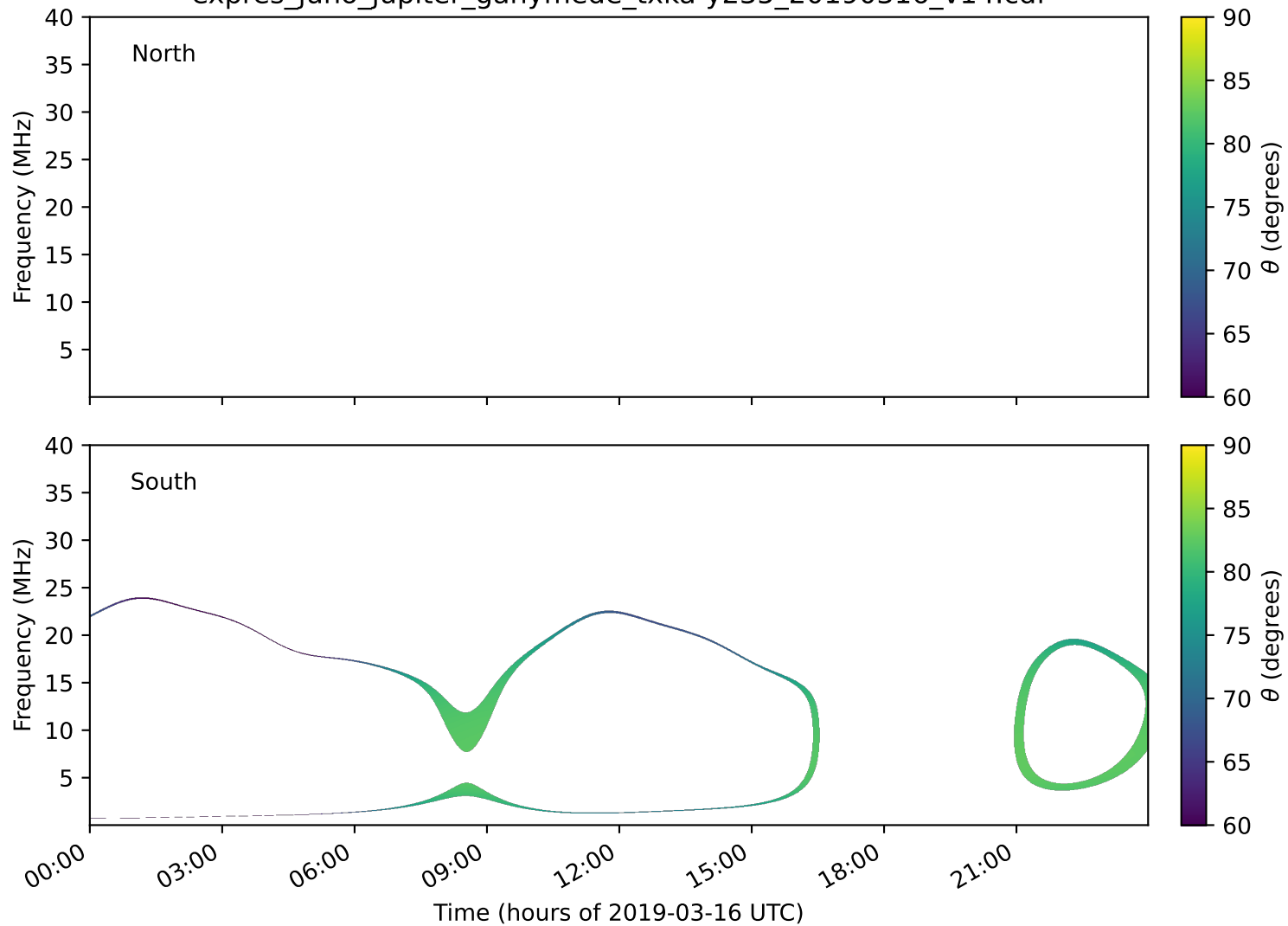
expres_juno_jupiter_ganymede_txka-y235_20190316_v14.cdf
