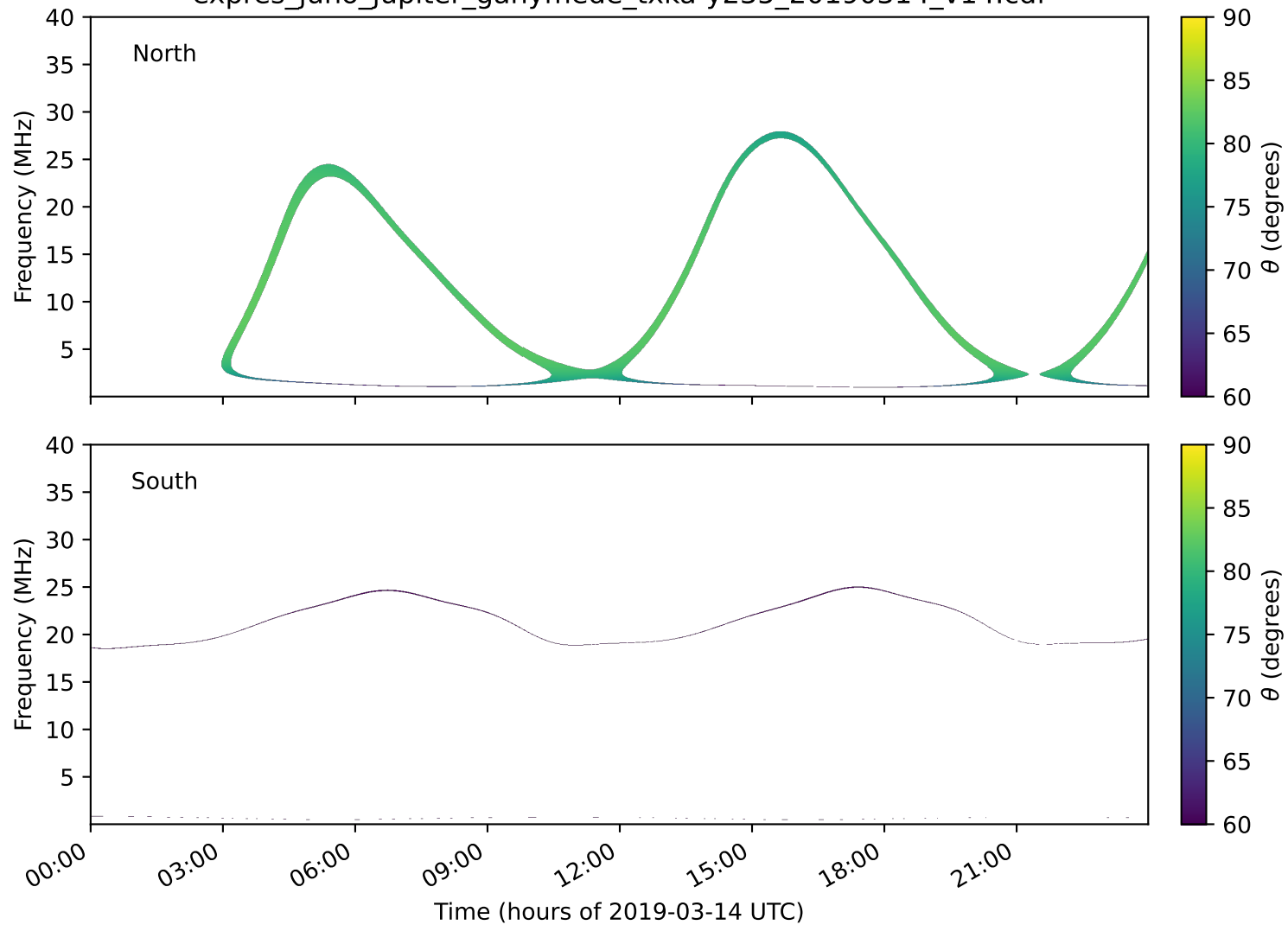
expres_juno_jupiter_ganymede_txka-y235_20190314_v14.cdf
