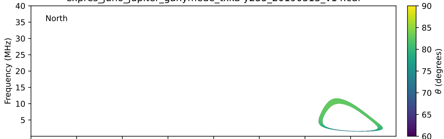
expres_juno_jupiter_ganymede_txka-y235_20190313_v14.cdf
