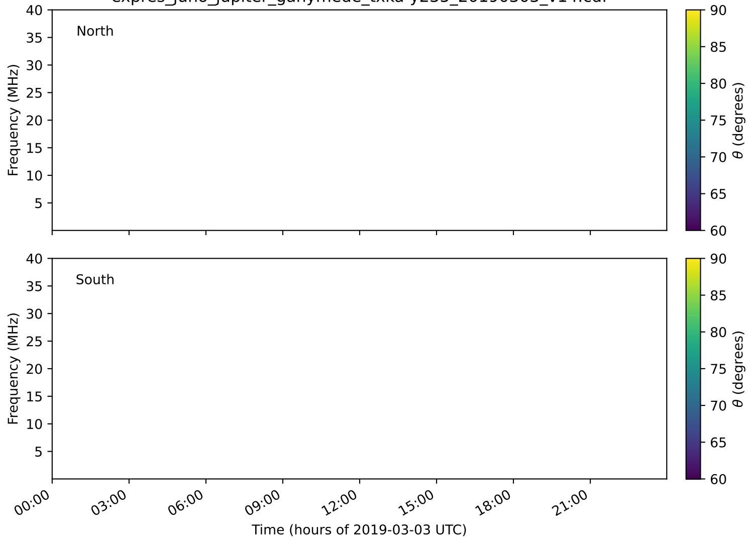
expres_juno_jupiter_ganymede_txka-y235_20190303_v14.cdf
