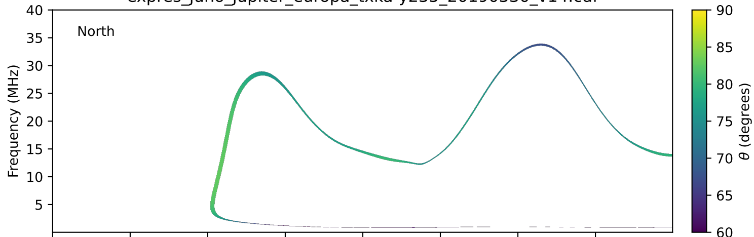
expres_juno_jupiter_europa_txka-y235_20190330_v14.cdf
