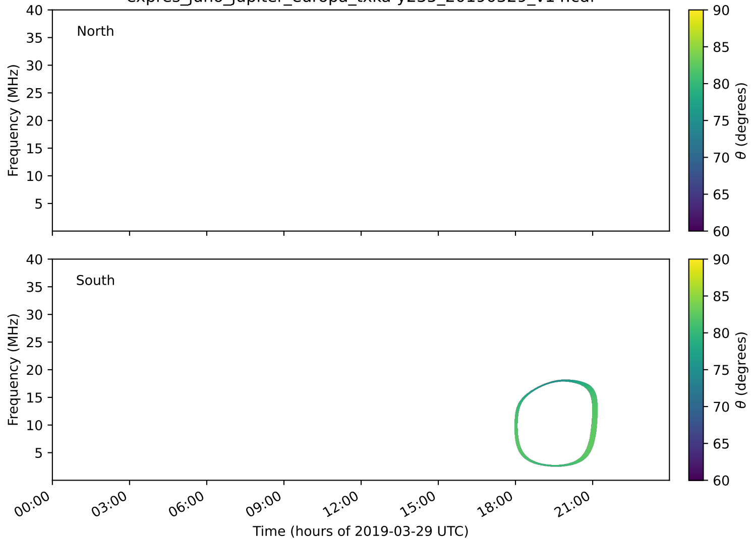
expres_juno_jupiter_europa_txka-y235_20190329_v14.cdf
